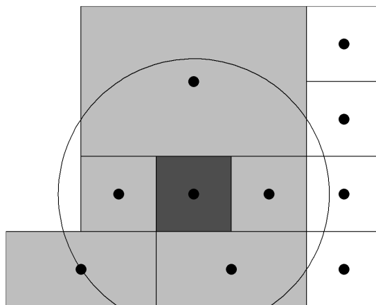
Figure 4: Distance-based neighbors (light) have centroids within a fixed radius of the reference cluster (dark). Clusters with centroids beyond this distance are not considered as neighbors (white) [21]
